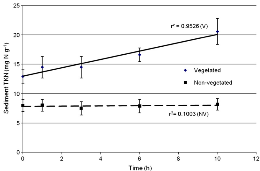
Fig. 5. Mean sediment TKN concentrations ( \text{mg N g}^{-1} ) for all sampling locations within the vegetated (solid line) and non-vegetated (dashed line) ditches through time.
